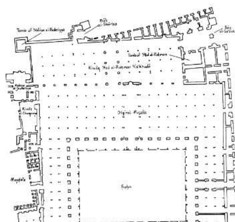
Figure 2: Plan of Al-Azhar Mosque Source: Rabbat 1996
