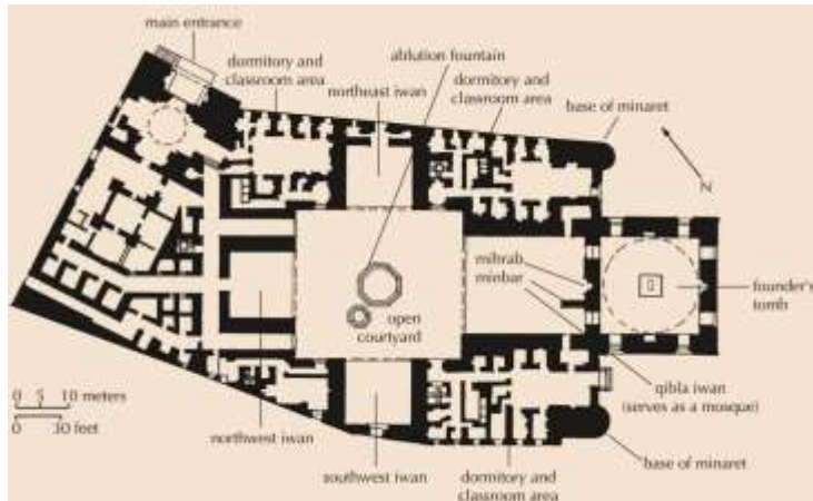
Figure 3-4: Great Mosque of Sultan Hasan, Cairo 1356-62 – Mamluk period. Source: Hillenbrand 2004
